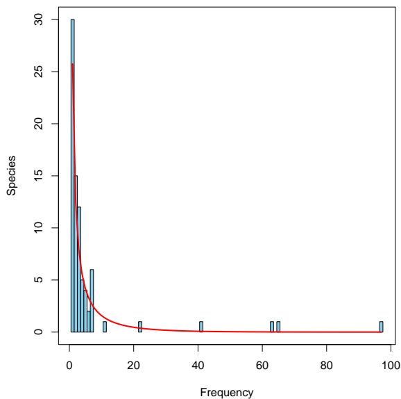
Figure 3: Fisher's log-series fitted to one randomly selected site (40).
