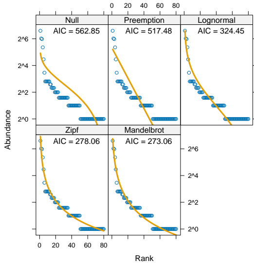
Figure 4: Ranked abundance distribution models for a random plot (no. 40). The best model has the lowest AIC.
